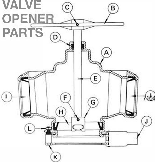
Ringlock Valve Opener Parts
