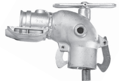
4" X 3" Elbow Valve Latch X RainTite™ Custom PN# 1012519
