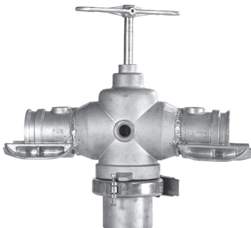
4" X 3" X 3" Tee Valve Ringlock X RainTite™ Custom PN# 1012583 and PN# 710109
