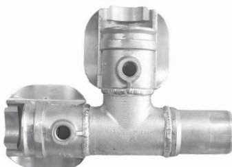
3" Line Tee Right Aluminum RainTite™ Custom PN# 1012525
